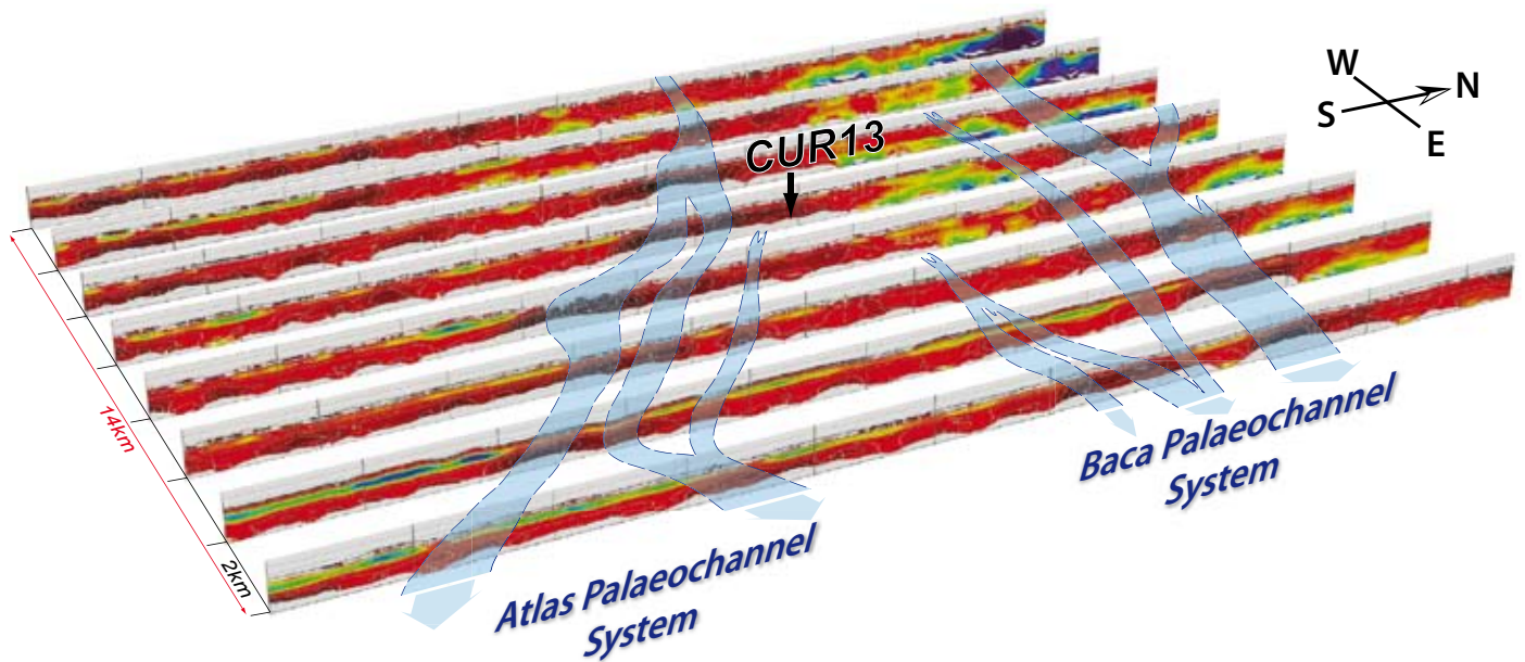
Figure 2 Stacked conductivity depth image (CDI) profiles within area of preliminary interpretation identifying palaeochannel systems and drillhole CUR13.
