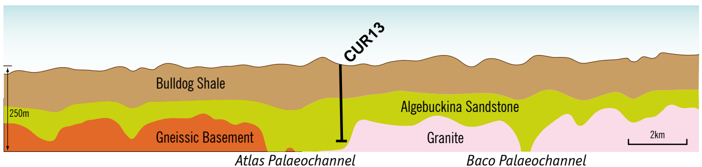
Figure 3 Interpreted geological cross-section displaying position of drillhole CUR13.
