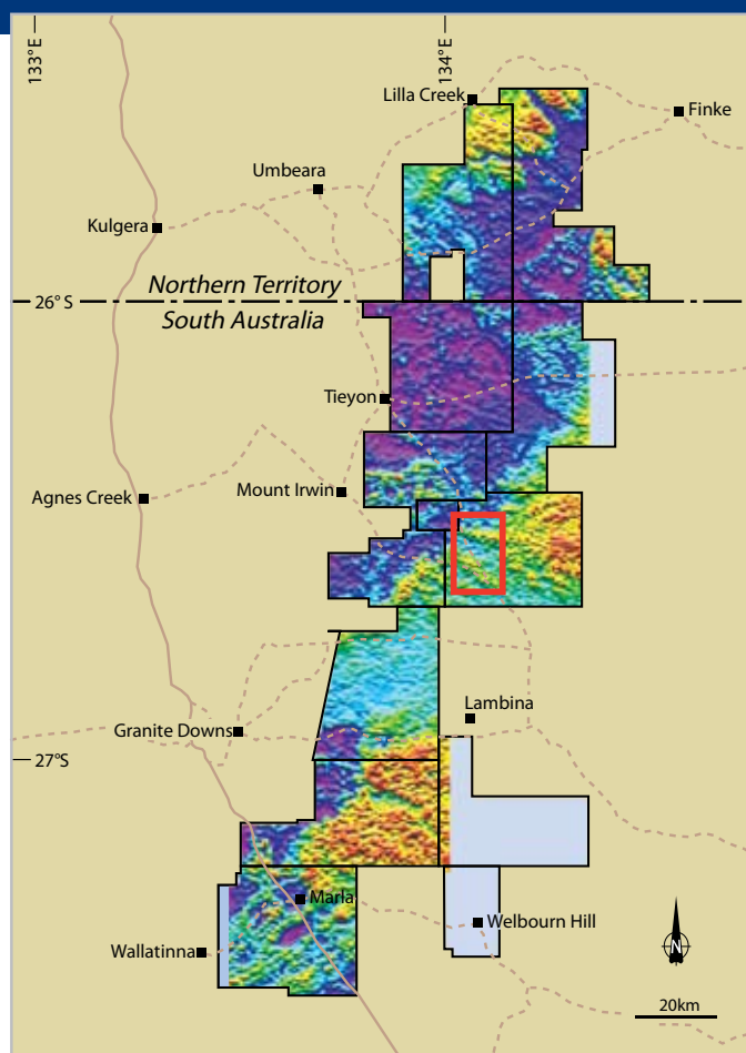
Figure 1 Abminga airborne electromagnetic image showing area of preliminary interpretation.
